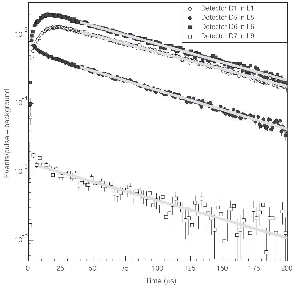
Fig. 9. Prompt response of MASURCA after a 1\text{-}\mu\text{s} neutron burst for the same criticality level (configuration III) in different positions of the MASURCA reactor. Locations: L5, core; L1 and L9, reflector; L6, shield.
