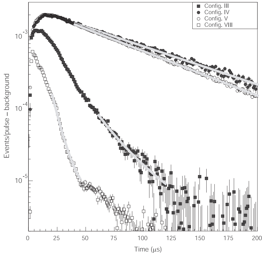
Fig. 8. Prompt response of MASURCA after a 1- \mu s neutron burst, observed by detector D1 placed in the reflector region (L1) for the different reactivity levels obtained in configurations III, IV, V, and VIII.
