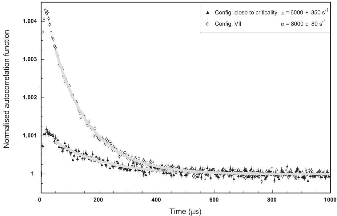
Fig. 13. Rossi distributions for two configurations.
