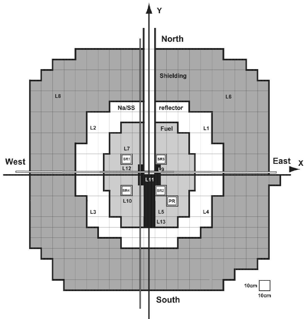
Fig. 4. XY cut of the MUSE-4 Reference critical configuration at the core median plane with measurement locations.
