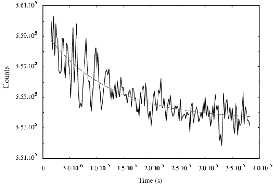
Fig. 14. Rossi- \alpha distribution for a subcriticality level of -3795 pcm (configuration VI).
