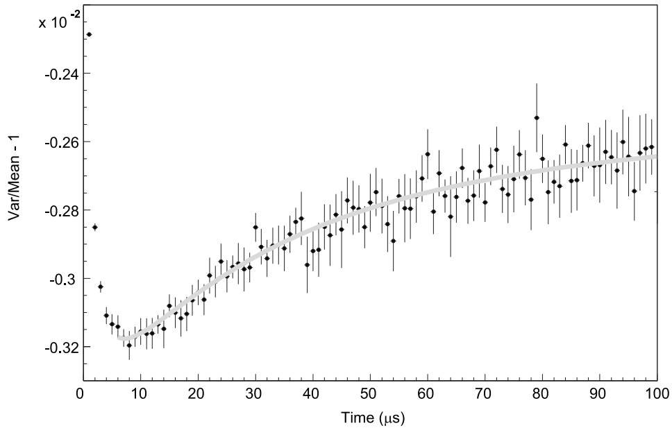
Fig. 16. Feynman- \alpha distribution for a subcritical configuration. The detector used is the same as in the Rossi- \alpha case (configuration VI).
