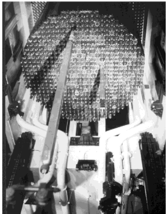
Fig. 2. MASURCA core loading from the bottom.
