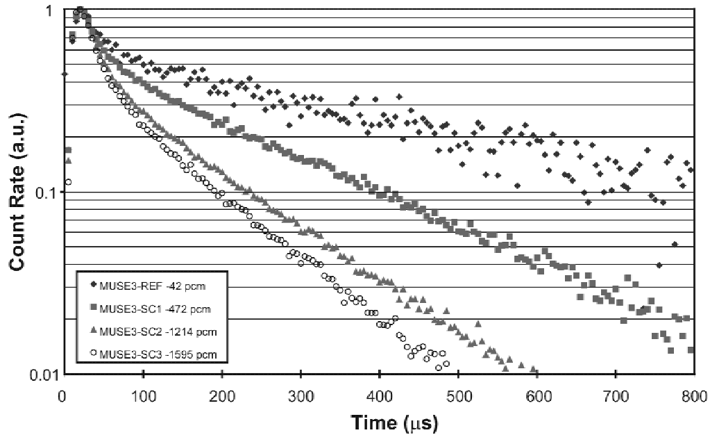
Fig. 1. Pulsed neutron source measurements in MUSE-3 for different subcritical levels.
