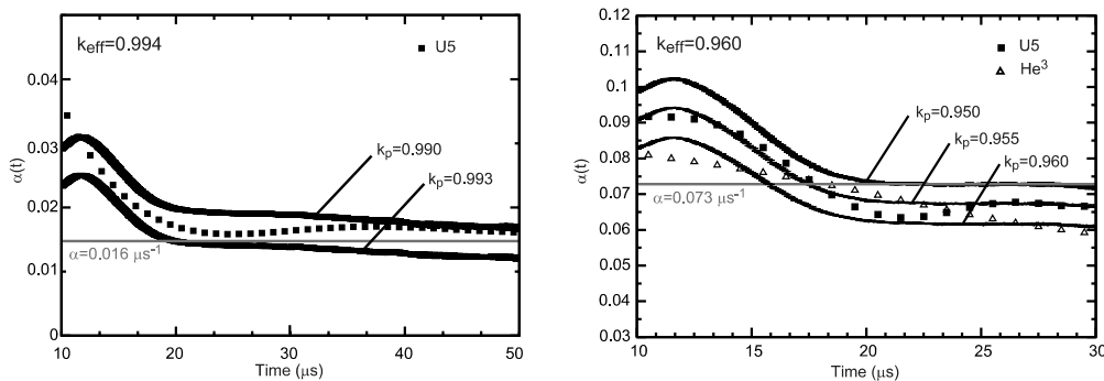
Fig. 11. Logarithmic derivatives of the fits of the experimental time spectra compared to several \alpha_{kp}(t) calculated by the proposed method.
