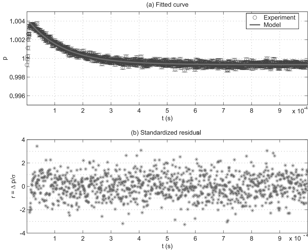
Fig. 12. Fit of the autocorrelation Rossi distribution.
