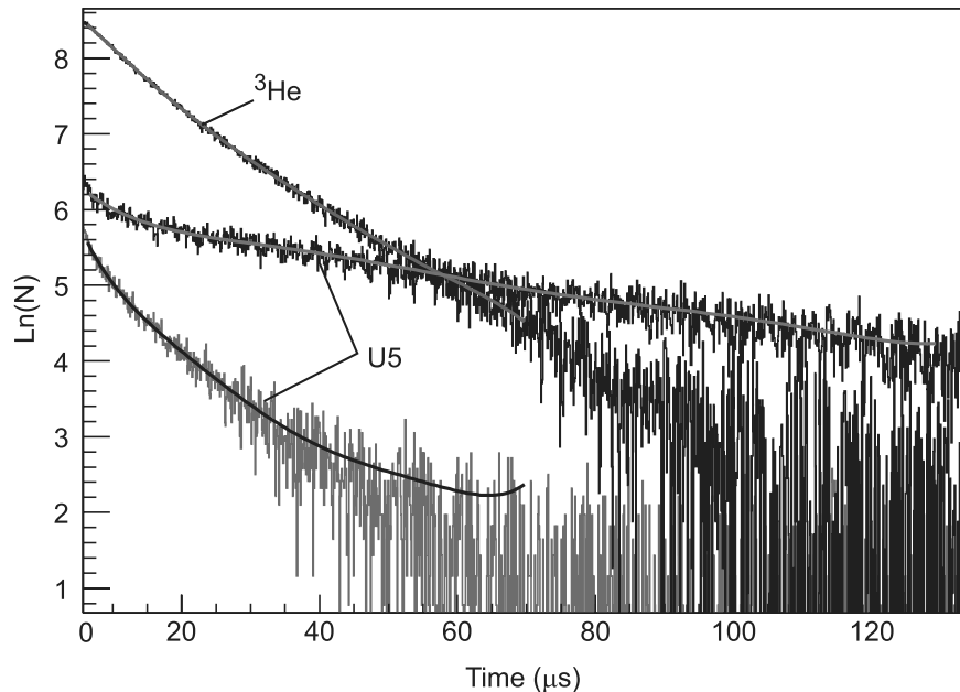
Fig. 10. \text{Ln}(N) time spectra obtained with a U5 FC (D12 in L12 for configuration III and in L10 for configuration V) and a ^3\text{He} detector (D13 in L13) in the fuel zone of MASURCA for two subcriticality levels k_{eff} = 0.995 and k_{eff} = 0.958 (configurations III and V). Plain curves are polynomial fits to the logarithm of the spectra.
