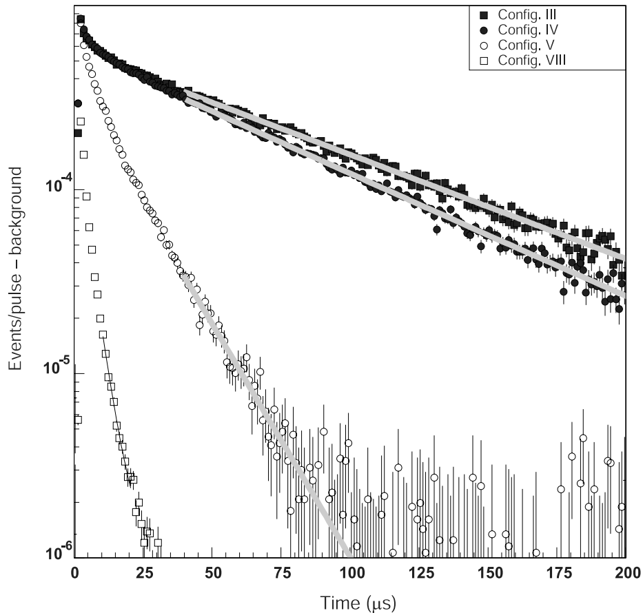
Fig. 7. Prompt response of MASURCA after a 1- \mu\text{s} neutron burst, observed by detector D5 placed in the core region (L5) for the different reactivity levels obtained in configurations III, IV, V, and VIII.
