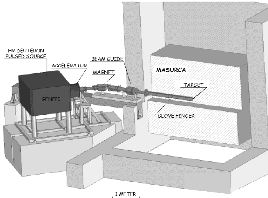
Fig. 3. The GENEPI accelerator coupled to MASURCA.
