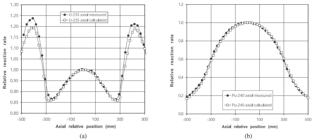
Fig. 6. Axial traverses thermal and threshold reaction rates: (a) ^{235}\text{U} and (b) ^{240}\text{Pu} .
