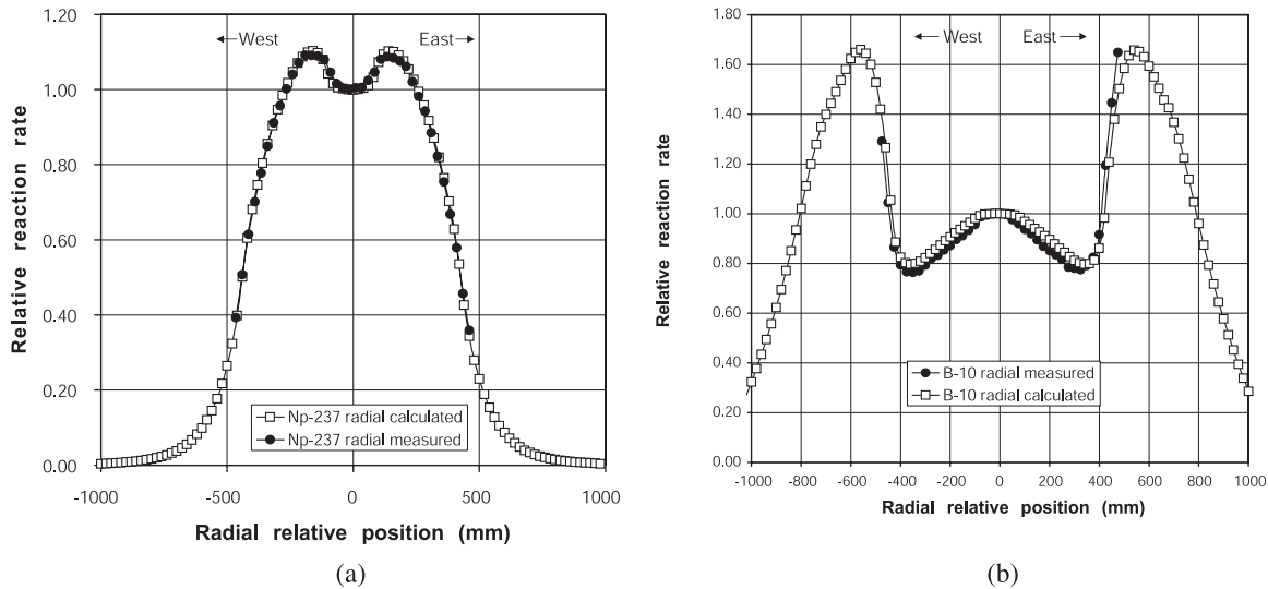
Fig. 5. Radial traverses thermal and threshold reaction rates: (a) ^{237}\text{Np} and (b) ^{10}\text{B} .
