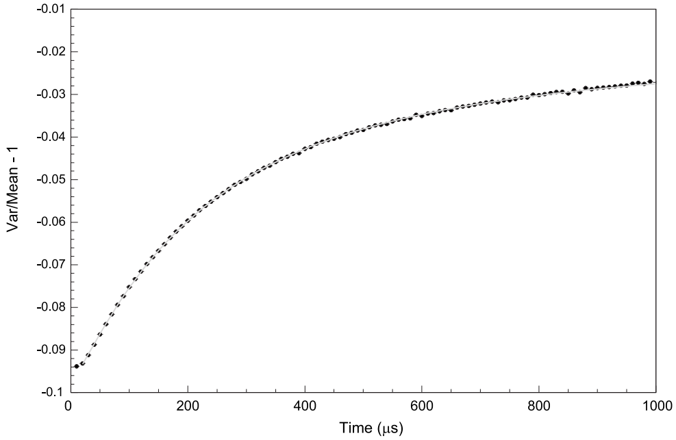
Fig. 15. Feynman- \alpha distribution for a configuration close to criticality situation. The detector used is the same as in the Rossi- \alpha case (configuration VII).
