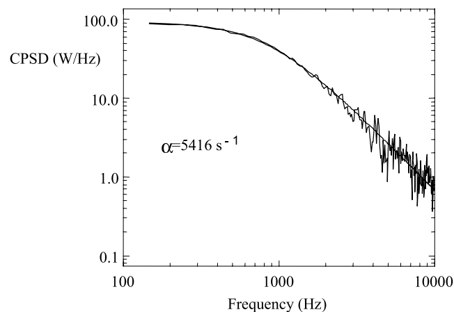
Fig. 17. The CPSD measured in continuous-current mode with high-efficiency detectors at positions L1 and L2. The \alpha value from the fit equals about 5416 \text{ s}^{-1} .
